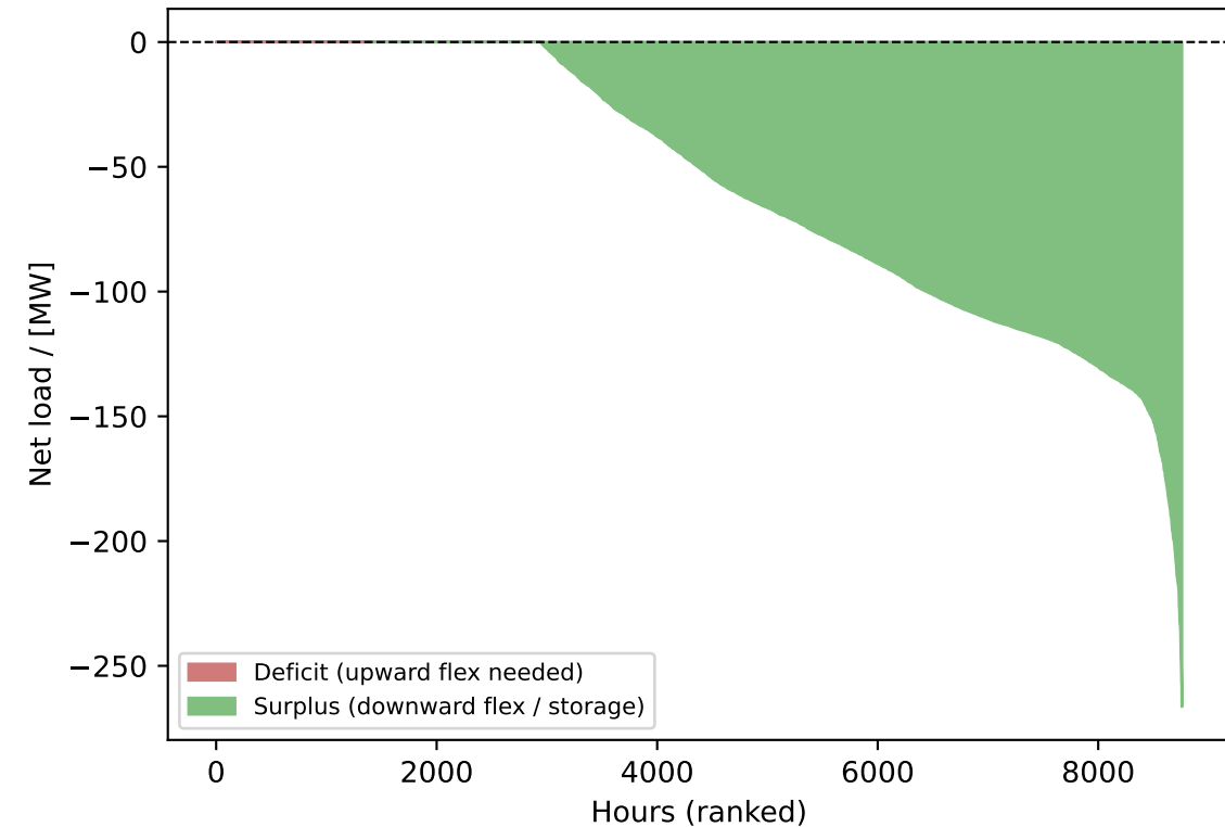
Heat Residual Load Duration Curve
