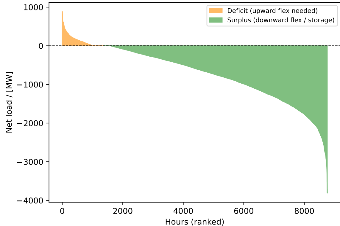
Electricity Residual Load Duration Curve
