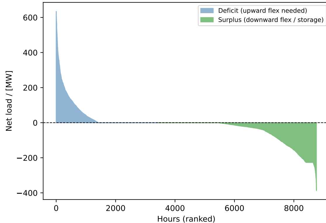
Hydrogen Residual Load Duration Curve
